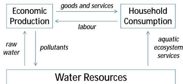
Figure 23: A schematic representation of the transactions between water resources, economic production and household consumption
