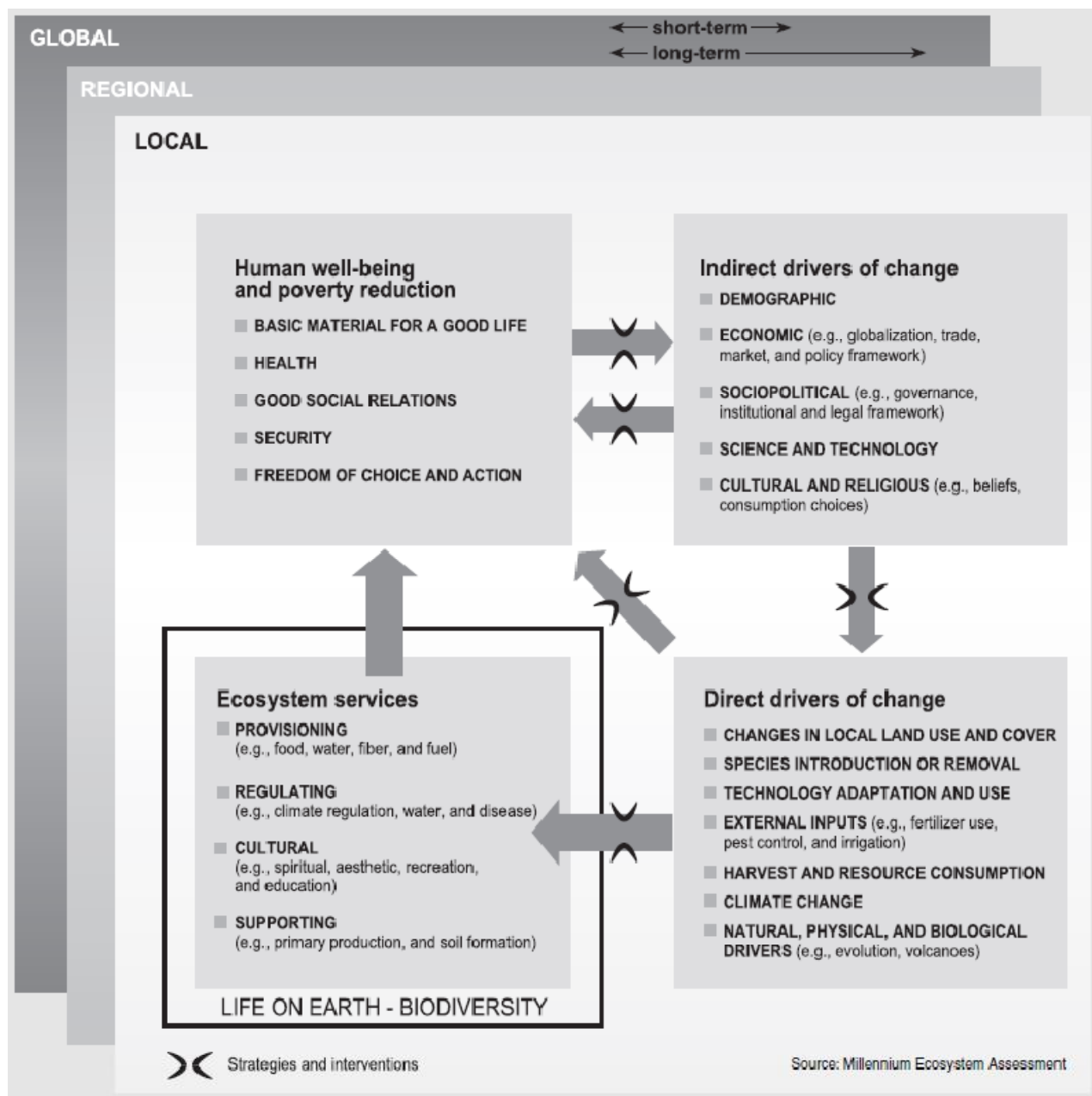
Figure 26: Conceptual framework of the Millennium Ecosystem Assessment (MEA 2003)
